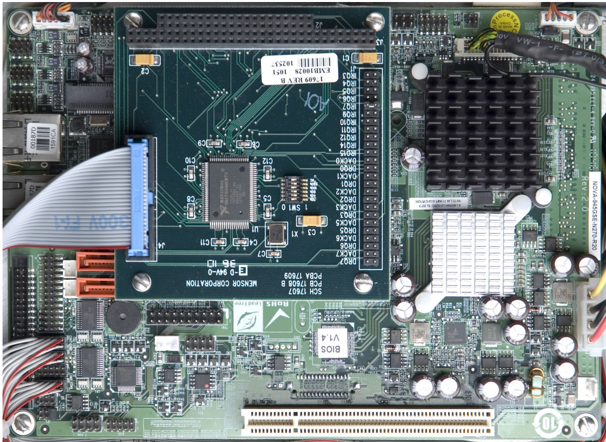
Figure 3.5 - Electrical Module
