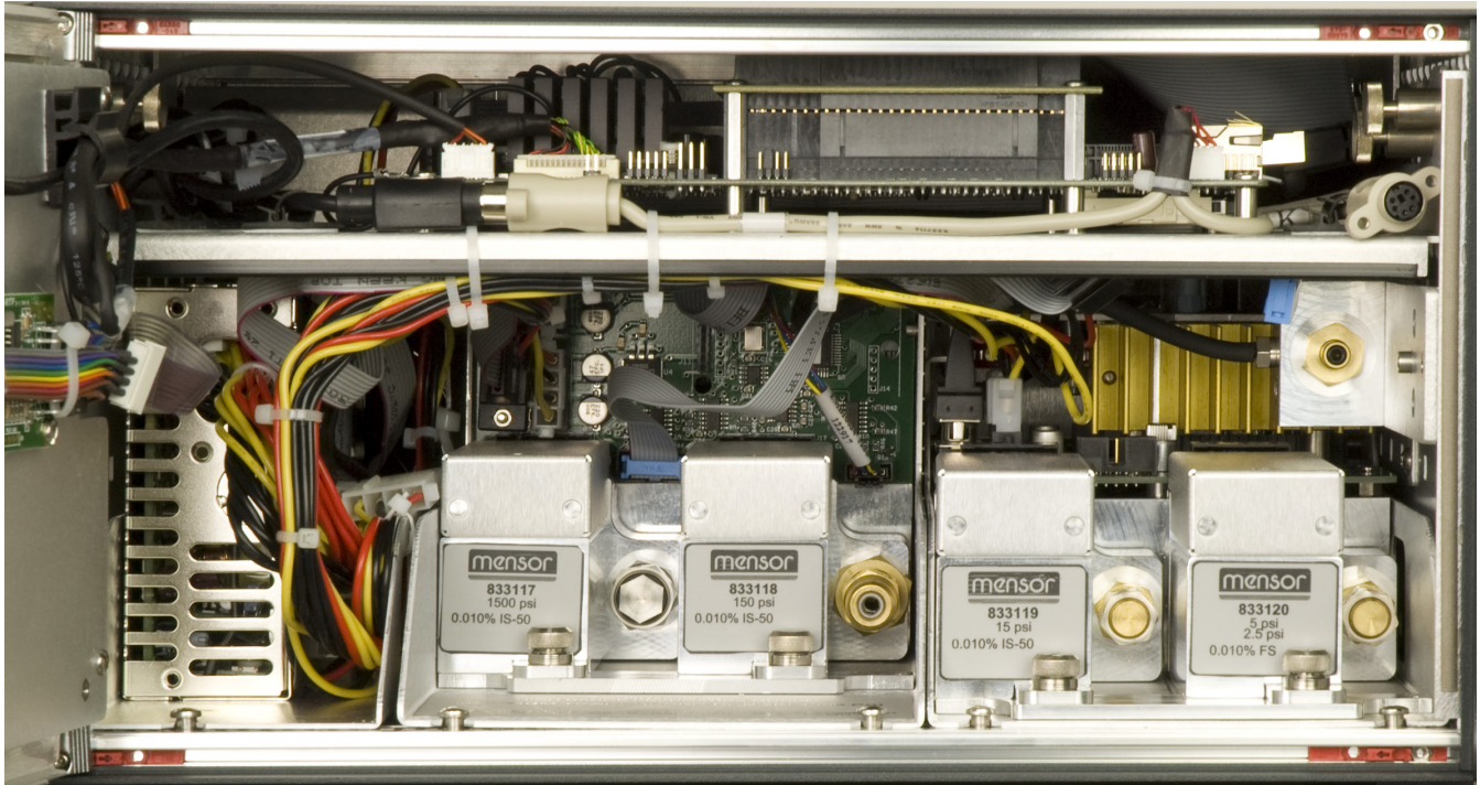
Figure 9.5B - Chassis Interior, Front View
